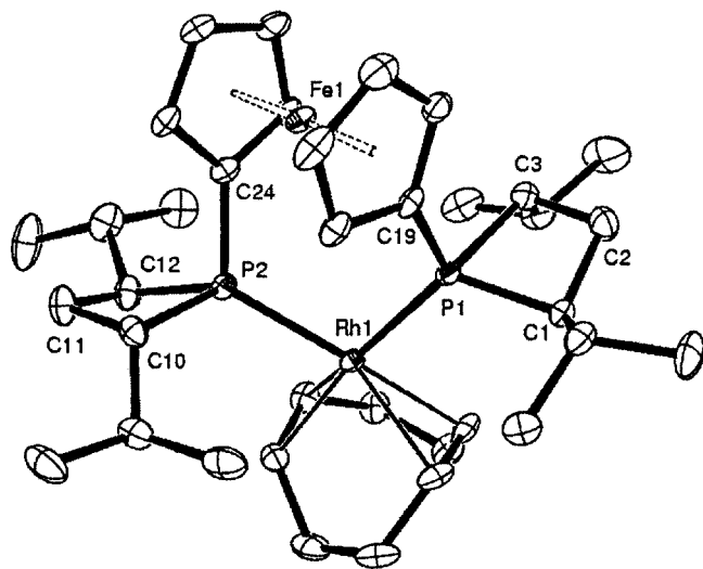
Figure 3. ORTEP drawing of the [(COD)Rh( 1c )OTf] complex 3c
