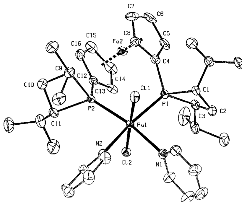
Figure 1. ORTEP drawing for the ruthenium complex 2c
