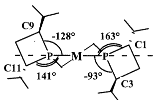
Figure 2. Coordination mode of the bis(phosphetano)ferrocene moiety in the ruthenium complex 2c
