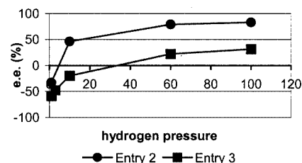
Figure 4. Plotting of data from Entries 2 and 3 in Table 4
